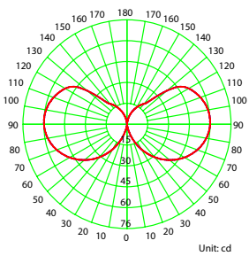
Luminous Intensity Distribution Curve - 2051.110.80L
