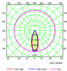
Luminous Intensity Distribution Curve - 6014.060.xXL
