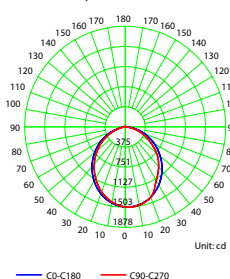
Luminous Intensity Distribution Curve - 5027.090.20L
