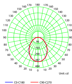
Luminous Intensity Distribution Curve - 1504.113.xFL
