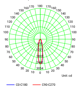
Luminous Intensity Distribution Curve - 1524.501.xXL
