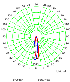
Luminous Intensity Distribution Curve - 1524.201.xXL
