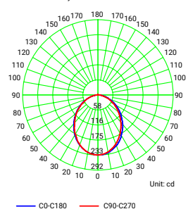
Luminous Intensity Distribution Curve - 2014.105.80L
