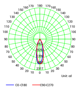
Luminous Intensity Distribution Curve - 2561.109.xPL
