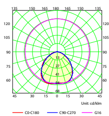
Luminous Intensity Distribution Curve - 2062.126.AFL
